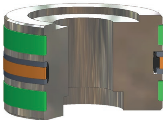
CT installed in Piston Gland
